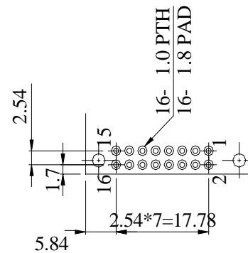
PIN DETAIL
